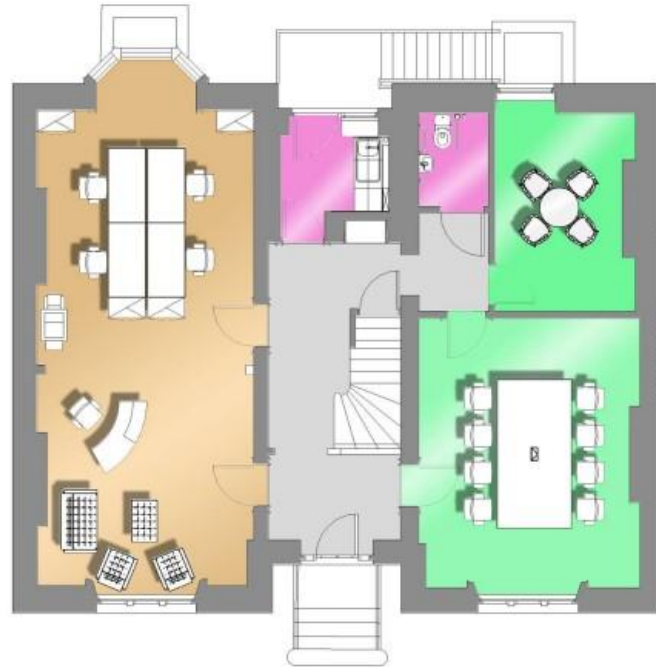
GROUND FLOOR LAYOUT, SCALE: 1 : 125
